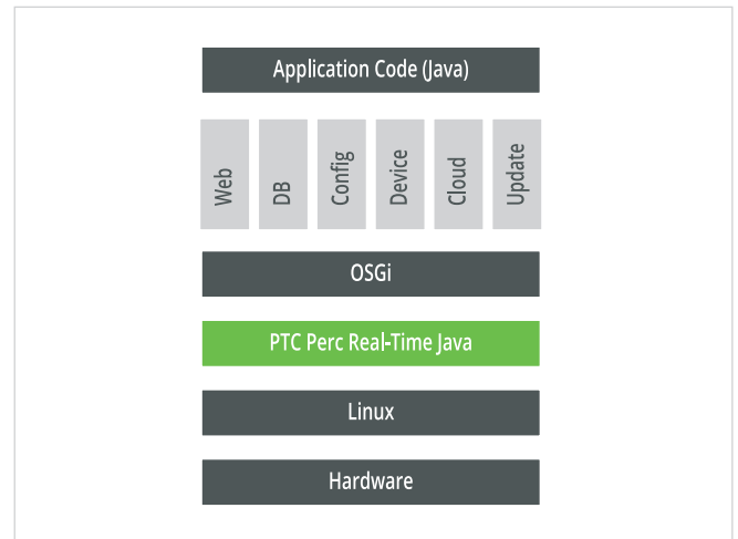
PTC Perc IoT Gateway Stack
