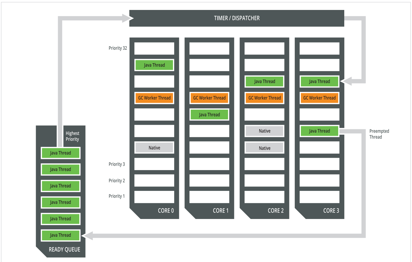
SMP Scheduling with PTC Perc
