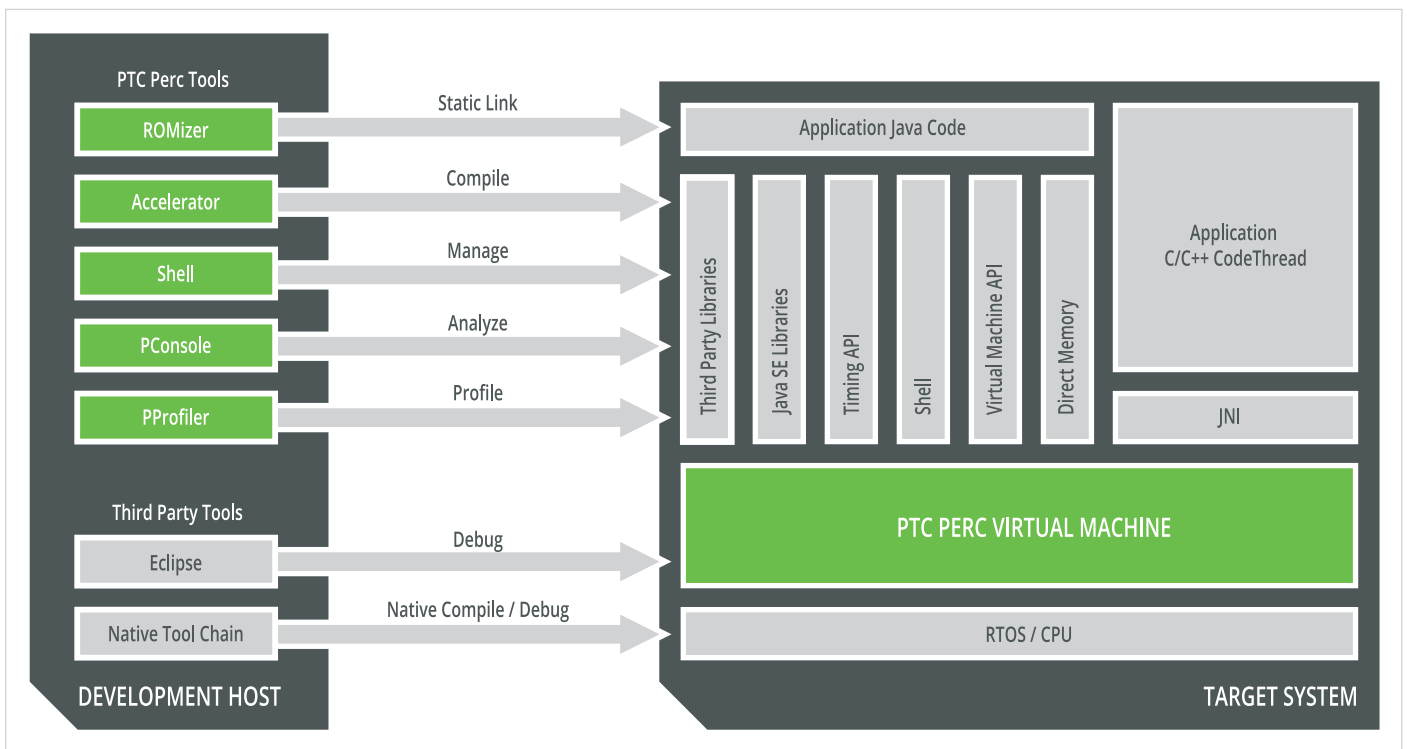
PTC Perc Toolchain
